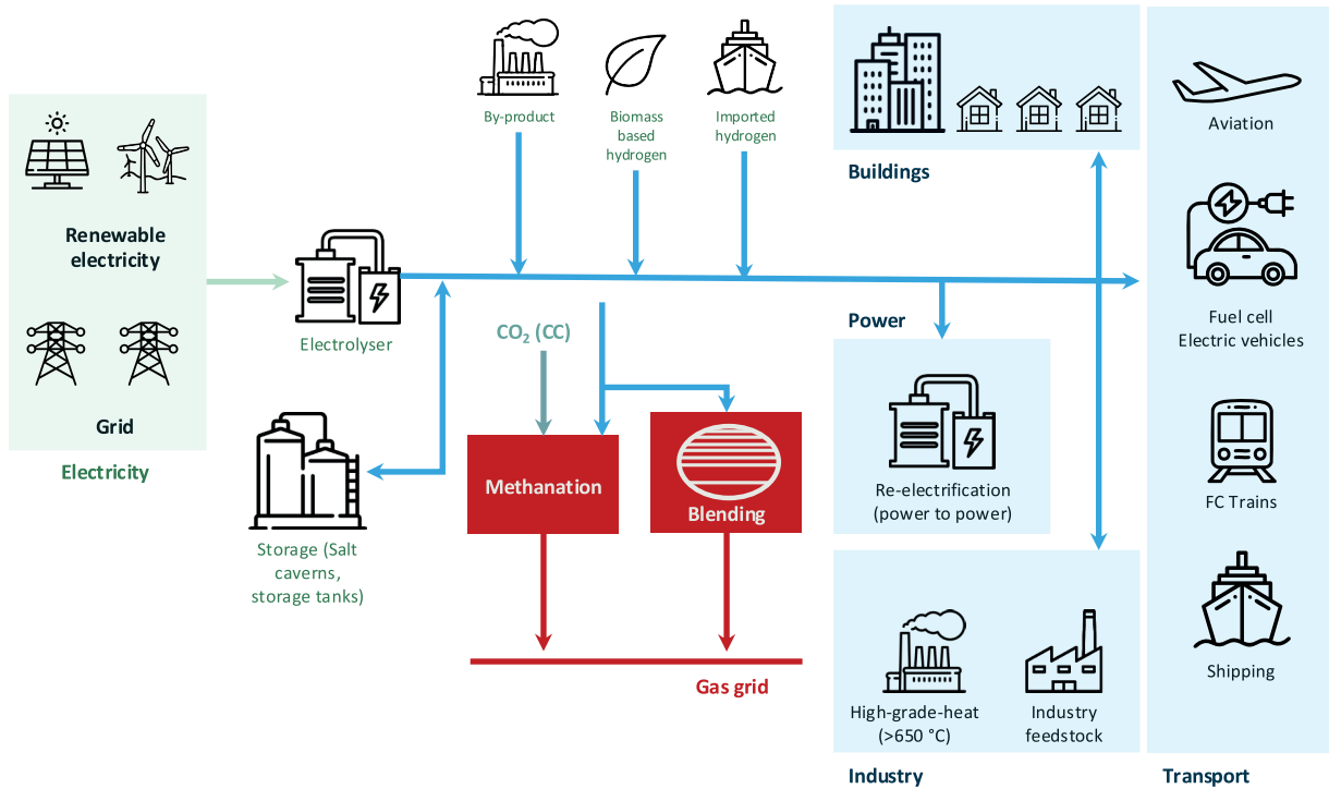
FIGURE 34 Coupling of the energy system sectors 163
